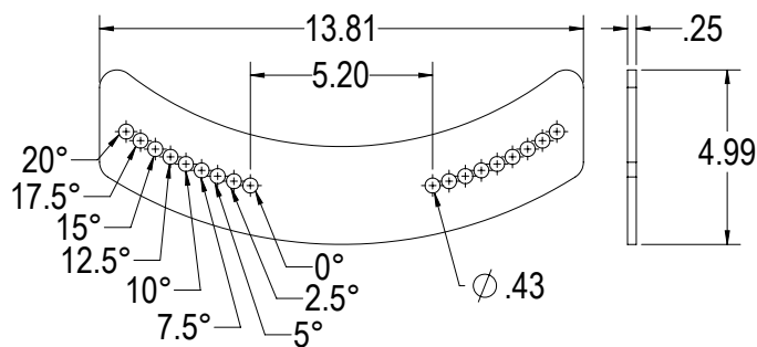
FRONT JOINER PLATE
