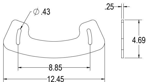
REAR JOINER PLATE
