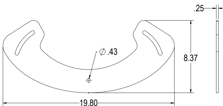
REAR JOINER PLATE
