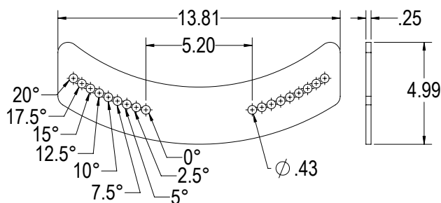
FRONT JOINER PLATE
