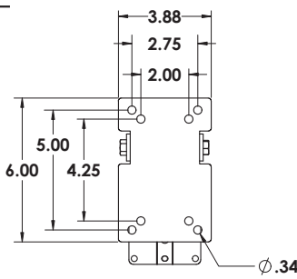
Speaker Adapter
