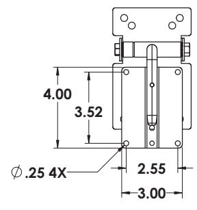
Wall Plate
